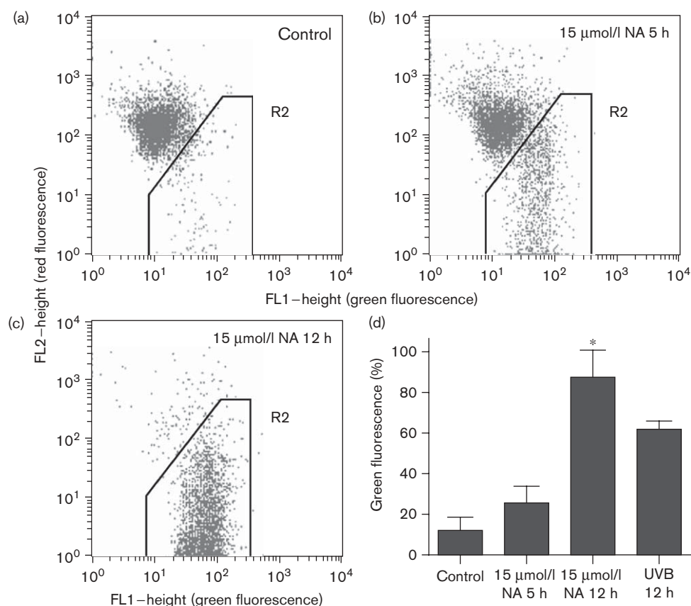
Naamidine A (NA) induced disruption of the mitochondrial membrane potential. (a) JC-1 (5,5',6,6'-tetrachloro-1,1',3,3'-tetraethylbenzimidazolocarbocyanine) analysis showing the formation of J-aggregates (red fluorescence) in A431 untreated control cells as assessed by fluorescence-activated cell sorter analysis. (b) A431 cells treated with 15 μmol/l NA for 5 h resulting in a 25% increase in green fluorescence (JC-1 monomer). (c) A431 cells treated with 15 μmol/l NA for 12 h resulting in a 97% increase in green fluorescence (JC-1 monomer). There is a clear shift in fluorescence from red (J-aggregates) to green (JC-1 monomers) after NA treatment for 12 h, which is indicative of the disruption of the mitochondrial membrane potential. (d) A431 cells treated with NA show an increase in cell populations displaying green fluorescence as compared with untreated control cells. NA induces a 20% green shift within 5 h of treatment. However, within 12 h of NA treatment, there is an 80% green shift. The t -test statistical analysis was used to compare differences in the percentage green fluorescence between untreated cells and cells treated with NA for 12 h, which yielded a P \leq 0.002 (*). UVB, ultra violet B.
